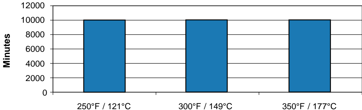
Chart #2 Static Shear of 3M™ Extreme Sealing Tape 4412N at Elevated Temperatures ASTM D-3654 (1" x 1", 100 grams, stainless steel) Panel Prep: 1 wipe 50/50 IPA/water; Prime with 3M™ Adhesion Promoter 111
